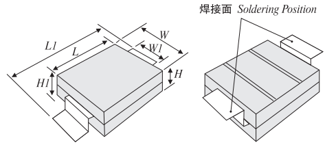
产品外折弯(Y型)外形及尺寸图 (图2) Fig.2 Structure and dimension of outward(Y style) Chip Zinc Oxide Varistor
