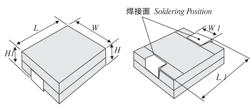
产品内折弯(C型)外形及尺寸图 (图1) Fig.1 Structure and dimension of inward(C style) Chip Zinc Oxide Varistor
